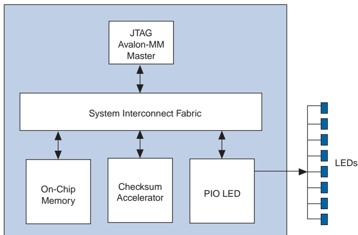
Figure 2-5. SOPC Builder System for Checksum Accelerator Example
