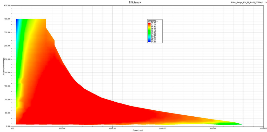
Figure 1. Efficiency map.
