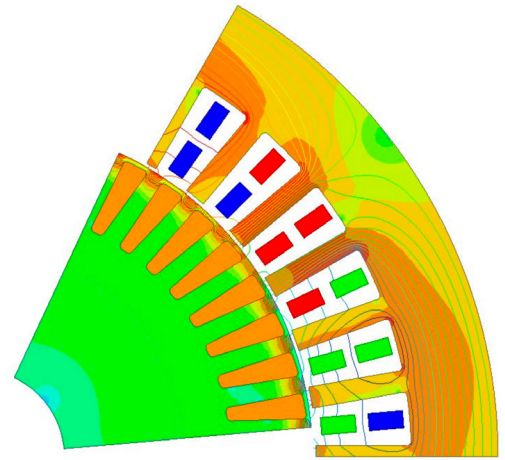
Figure 4. Induction machine.
